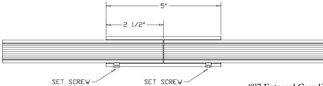
#87 External Coupling
