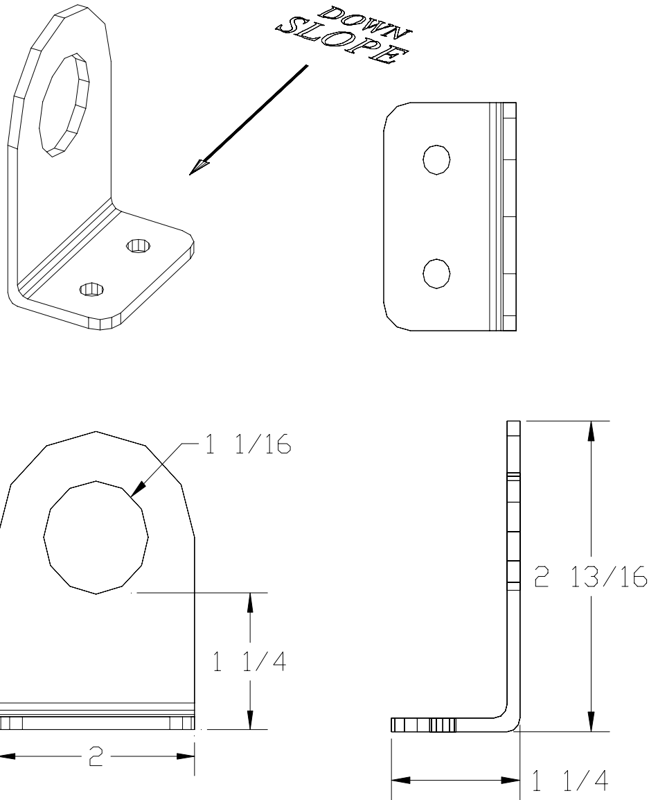
#245 1-Pipe Style Snowguard Bracket for Through-fastened Metal Roof Applications
